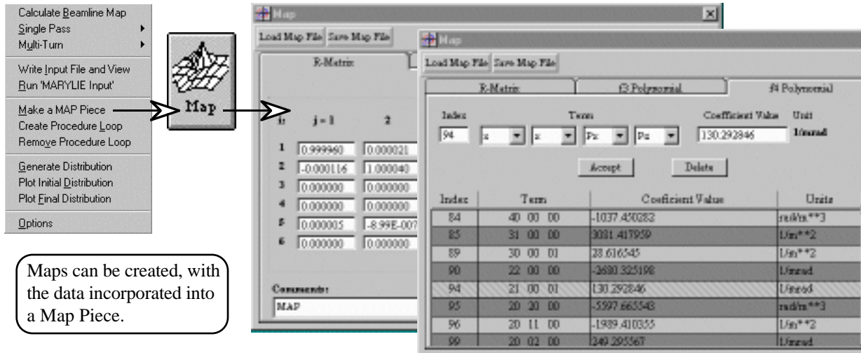
Figure 4. A map can be generated for a group of elements and the data entered automatically into a Map Piece.
