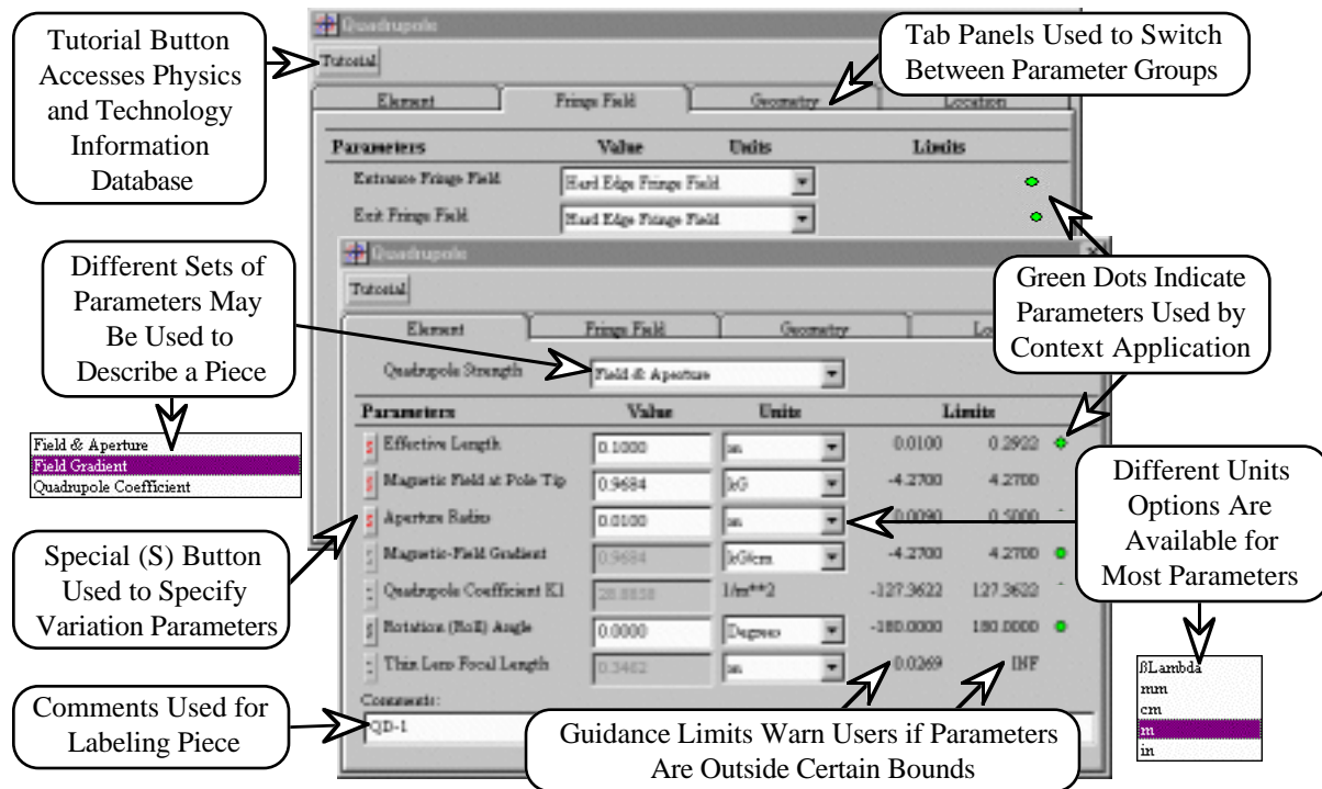
Figure 2. Example of Piece Window (left) and Alias Window (right) for editing parameters of a magnetic bend element.
