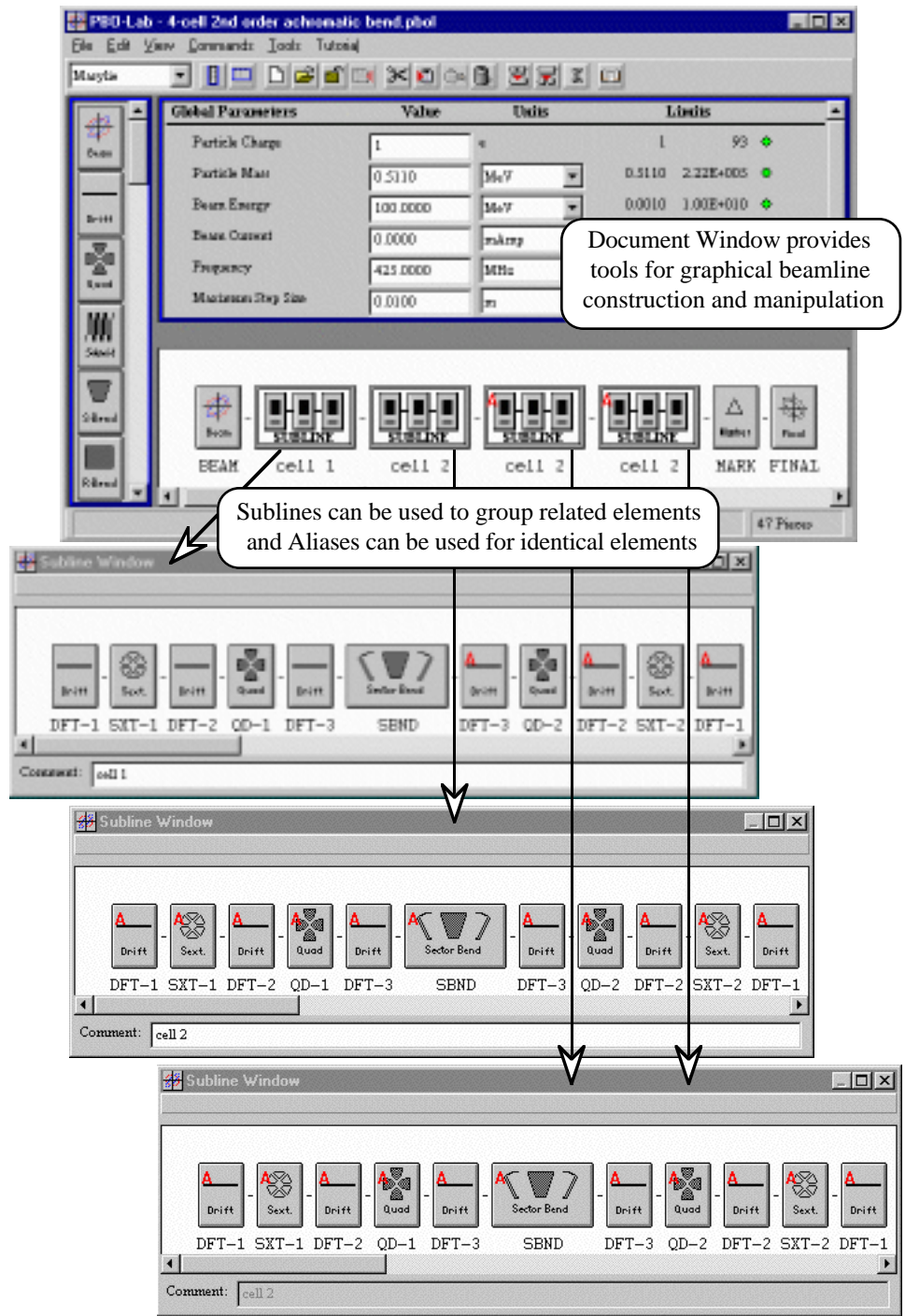
Figure 1. Example Document Window and three Subline Windows of the graphic user interface for MARYLIE.
