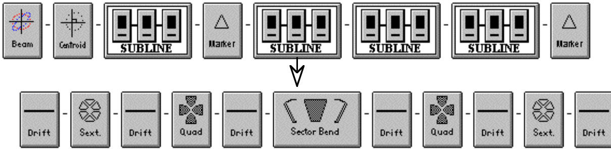
Figure 1. Icon image (from a PBO Lab Document Window) illustrating the four-cell layout (each cell represented by a Subline) of the quarter-wave transformer and the basic elements comprising one of the four identical cells.
