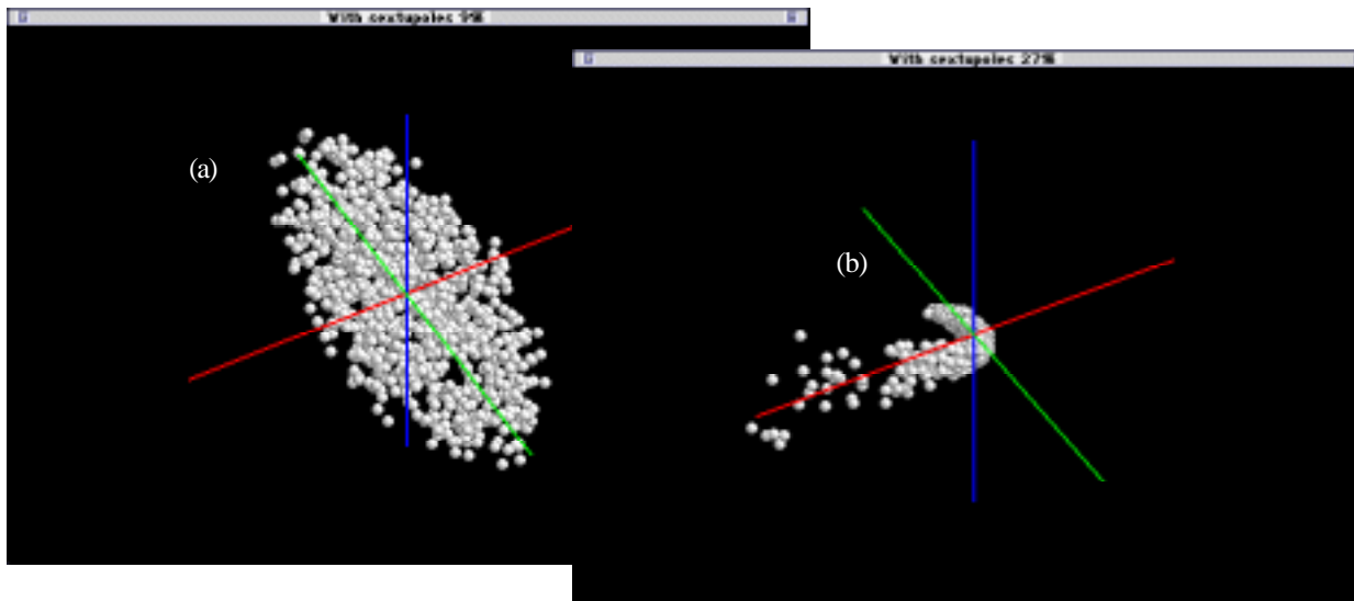
Figure 6. Snapshots of exit distributions of the corrected achromat, for initial beams with momentum spreads of (a) 9% and (b) 27%. The view orientations correspond to that of Figure 5(c), but are not to the same scale.
